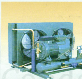
Condensing Units with Semi Hermetic Compressors of all brand as per the Customer's request & suitability of the requirement. Air Cooled & Water Cooled.
